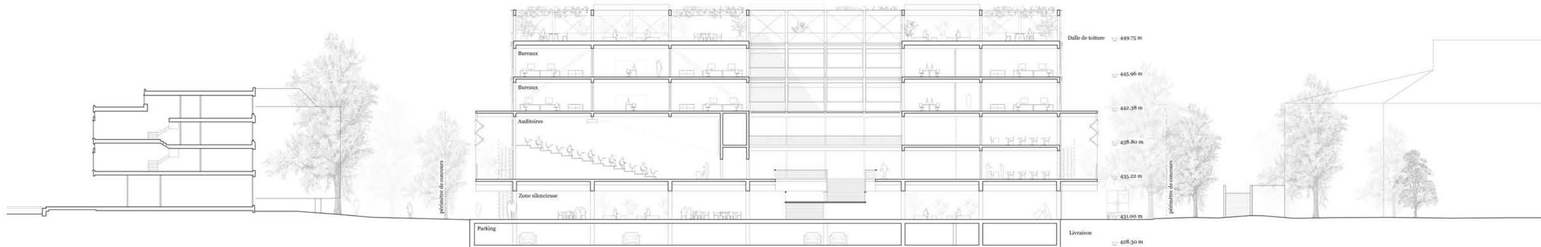
Section transversale _ 1:200
